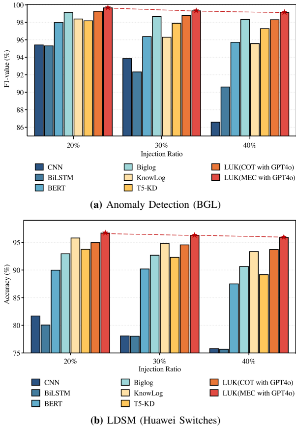
Fig. 7. Results on different synthetic datasets of unstable log.
