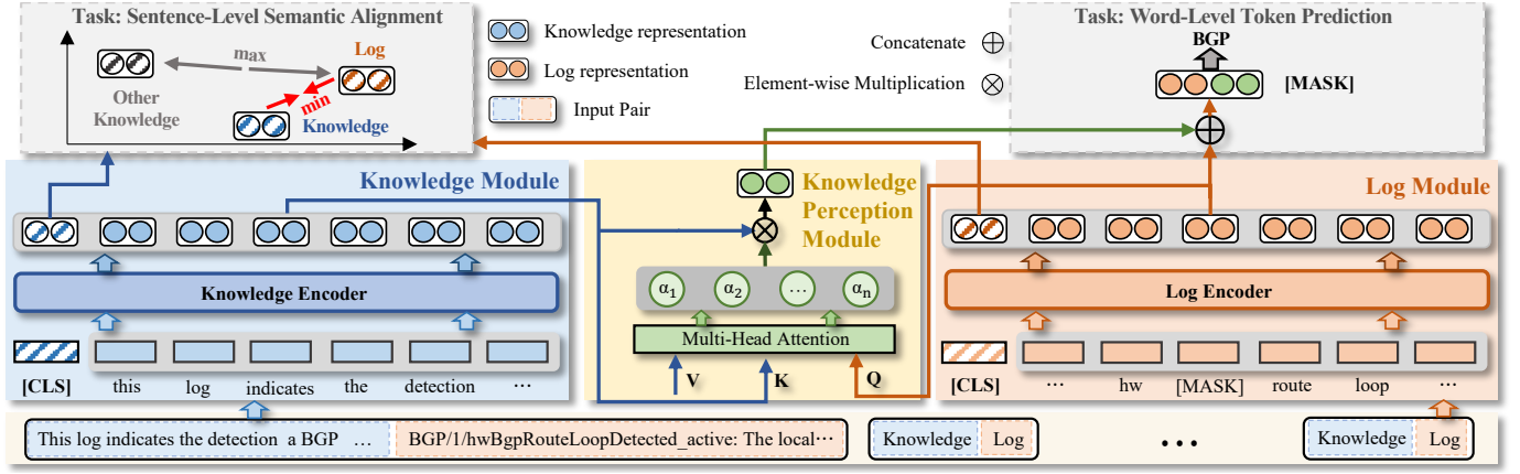
Fig. 5. The overview of LUK pre-training framework. LUK includes two novel pre-training objectives on word level and sentence level. The word-level object is designed from the perspective of domain token understanding, while the sentence-level objective is designed from overall semantic alignment.
