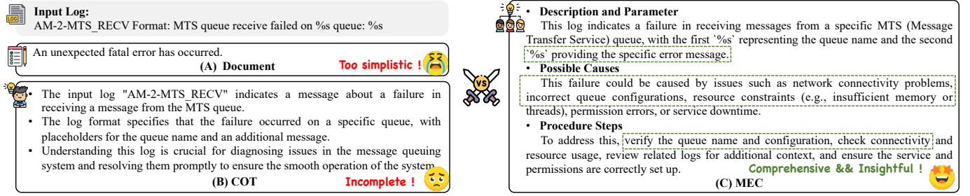
Fig. 13. Example of knowledge generated by GPT-4o and retrieved from documentation.
