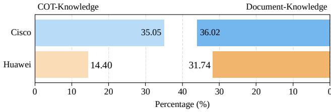
Fig. 14. Proportion of unsatisfactory knowledge, where we employ the evaluation criteria of the MEC framework to evaluate the knowledge.
