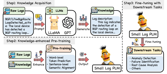
Fig. 2. Conceptual overview of LUK.
