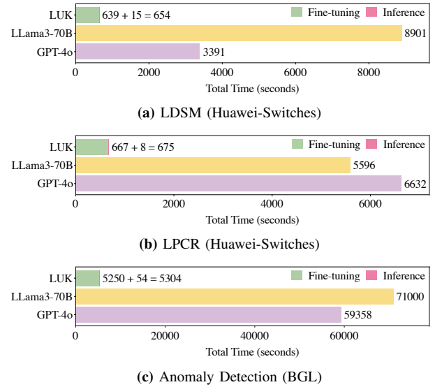
Fig. 9. Time expense of different models during reasoning.
