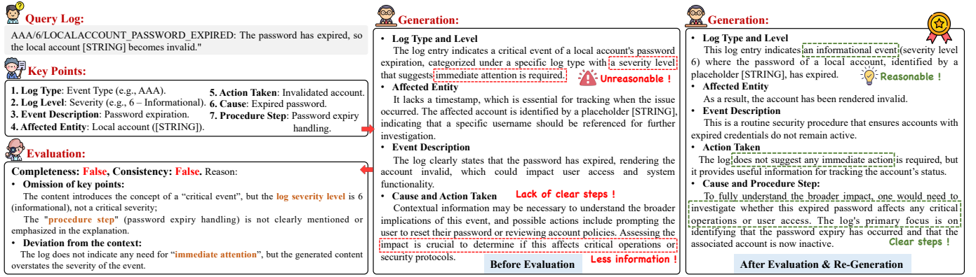
Fig. 11. A complete workflow of the MEC framework to construct knowledge.
