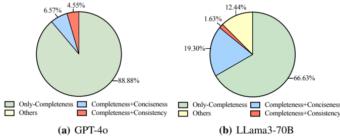
Fig. 12. Distributions of error categories in unsatisfactory knowledge.
