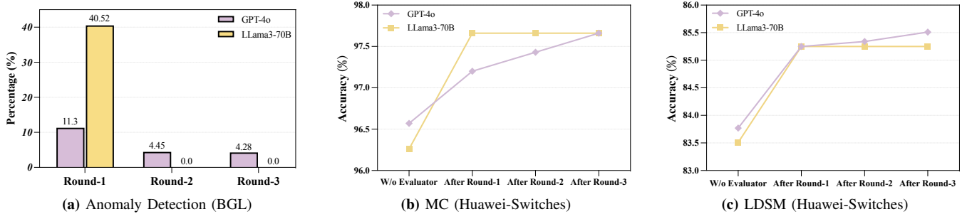
Fig. 10. Figure (a) shows the proportion of unsatisfactory knowledge in each iteration. Figure (b) and (c) show the results of the refined knowledge based on the evaluation feedback each time.
