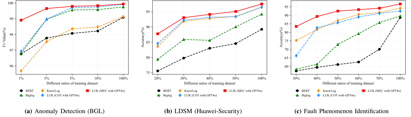
Fig. 8. Results on different ratios of the training dataset.
